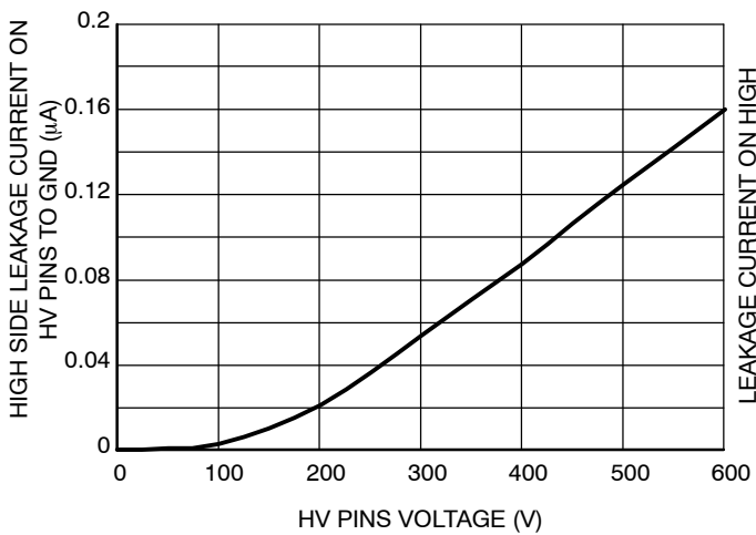
Figure 36. Leakage Current on High Voltage Pins (600 V) to Ground vs. V BRIDGE Voltage (V BRIDGE = V BOOT = V DREV_HI )
