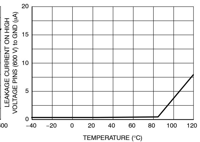
Figure 37. Leakage Current on High Voltage Pins (600 V) to Ground vs. Temperature (V BRIDGE = V BOOT = V DREV_HI = 600 V)
